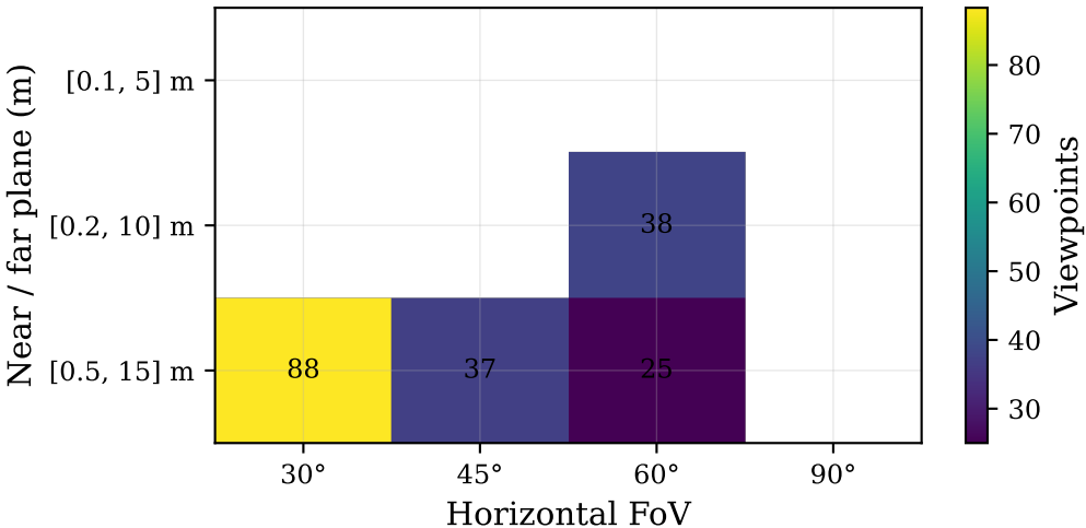
Viewpoints selected (Duke, targeted_50, 95% cov)
