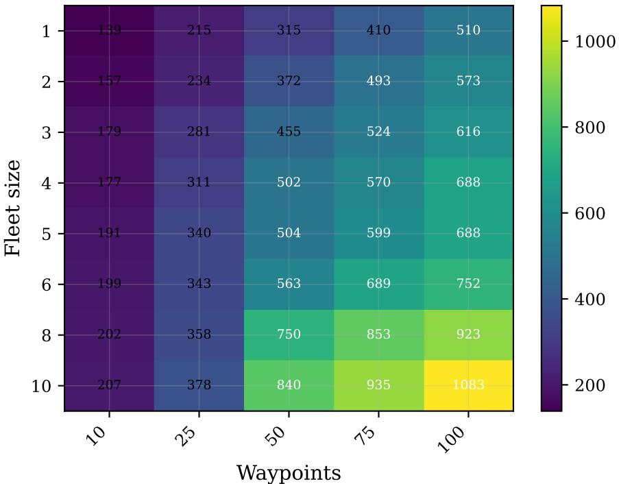
Total route cost (m)
