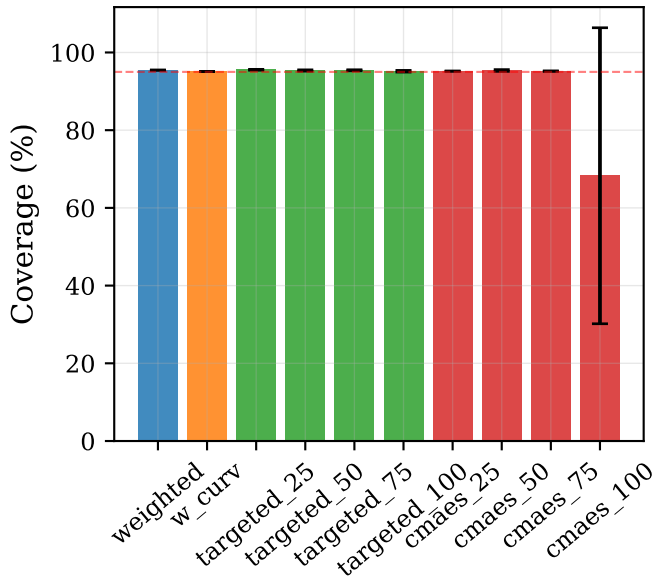
Coverage (wolf0)
