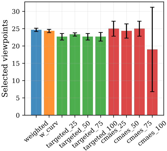
Viewpoints (wolf0)
