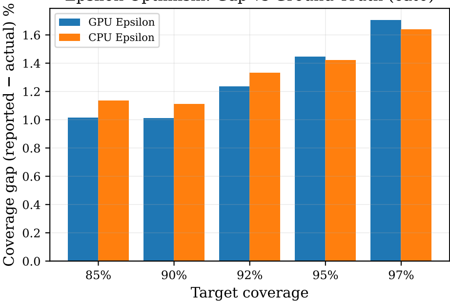
Epsilon Optimism: Gap vs Ground Truth (cat0)
