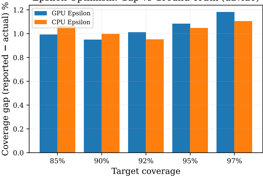
Epsilon Optimism: Gap vs Ground Truth (david0)
