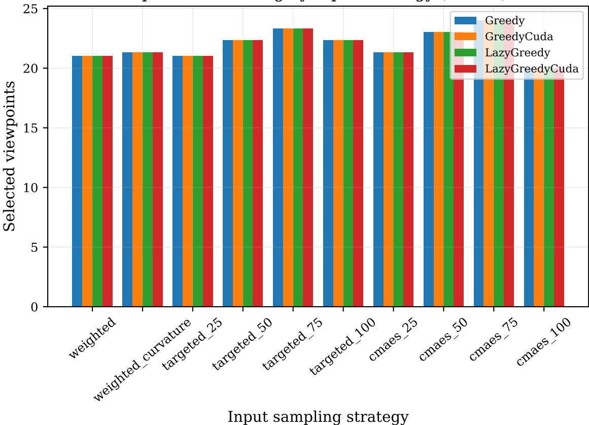
Optimizer Ranking by Input Strategy (david0)
