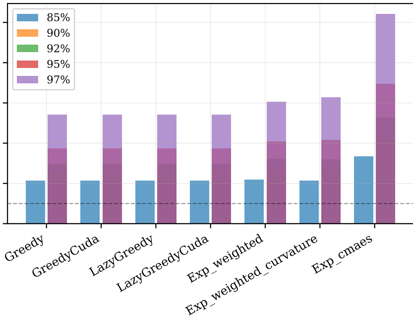
Optimality Ratio (duke_of_lancaster)
