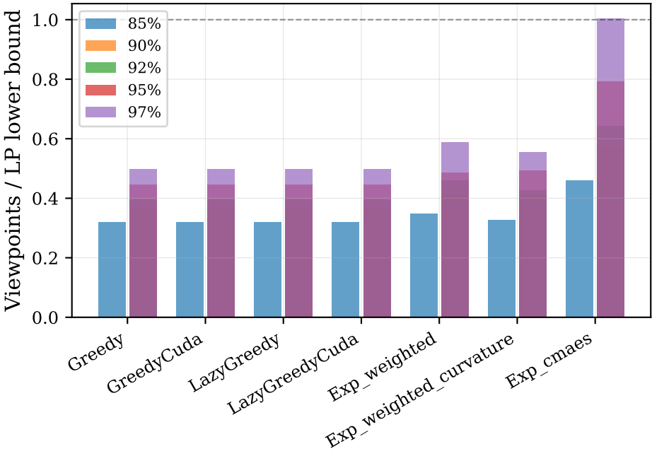
Optimality Ratio (wolf0)
