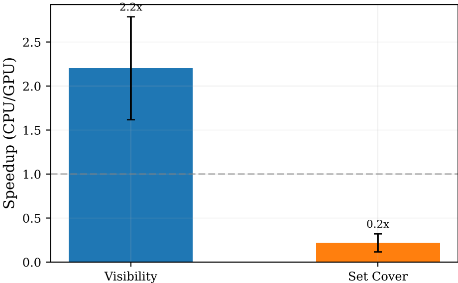
Per-Component GPU Speedup
