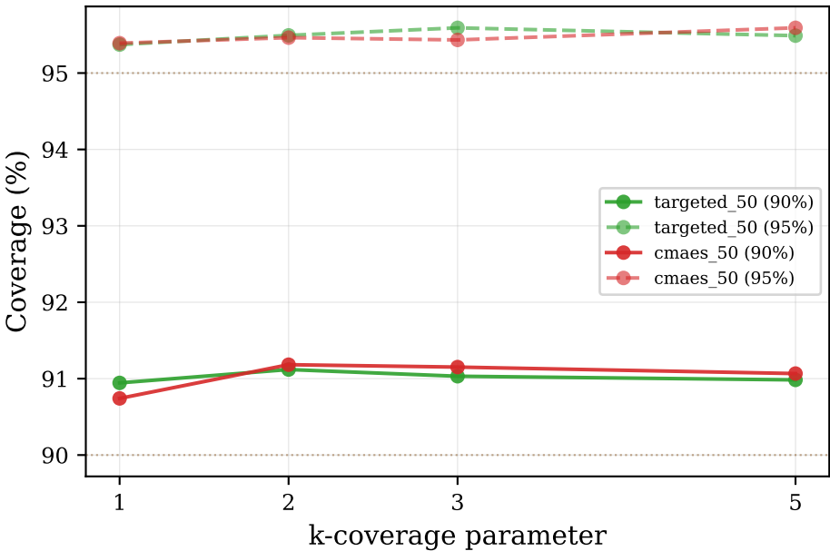
Coverage vs k-Coverage (N=1500·k, TOSCA)
