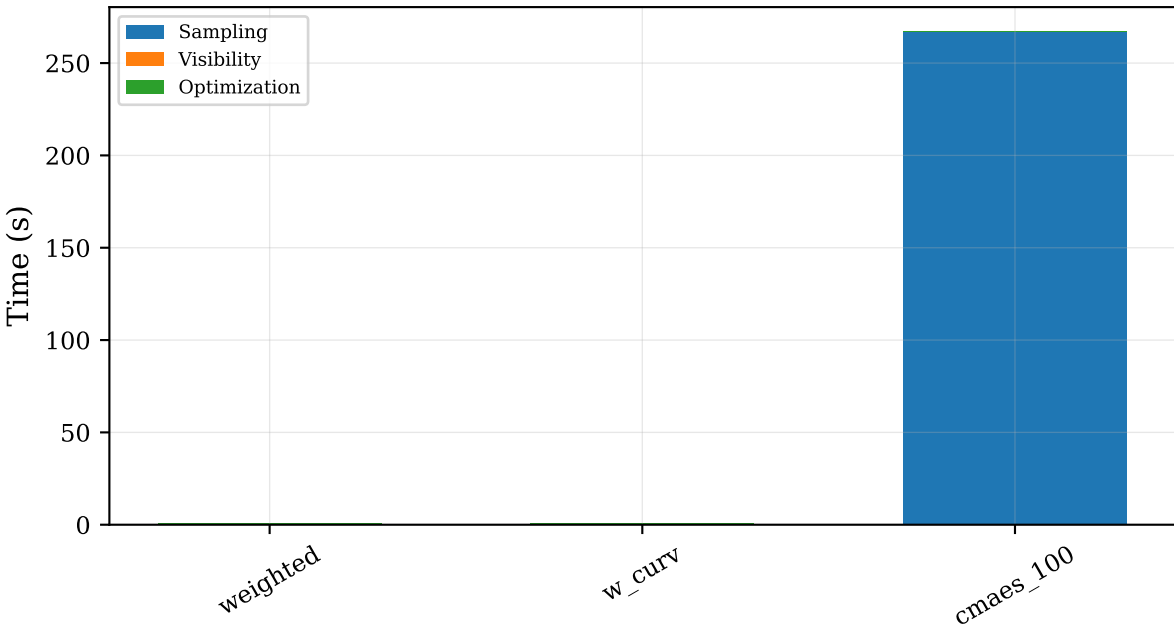
Per-Stage Timing (mean across models)
