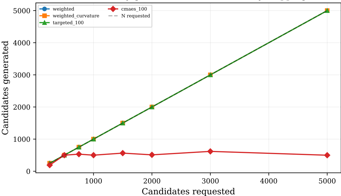
Actual Candidates Generated (CMA-ES may generate fewer due to early stopping)
