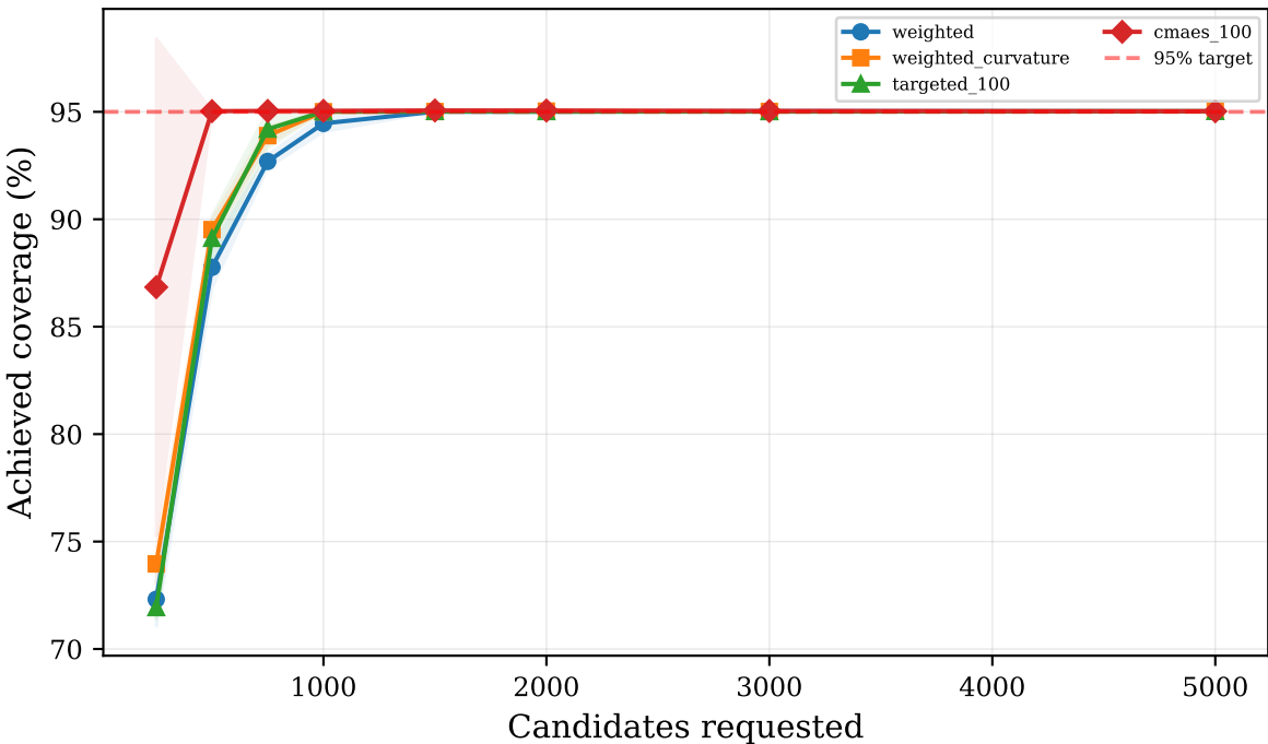
Coverage vs. Candidate Count — All Strategies
