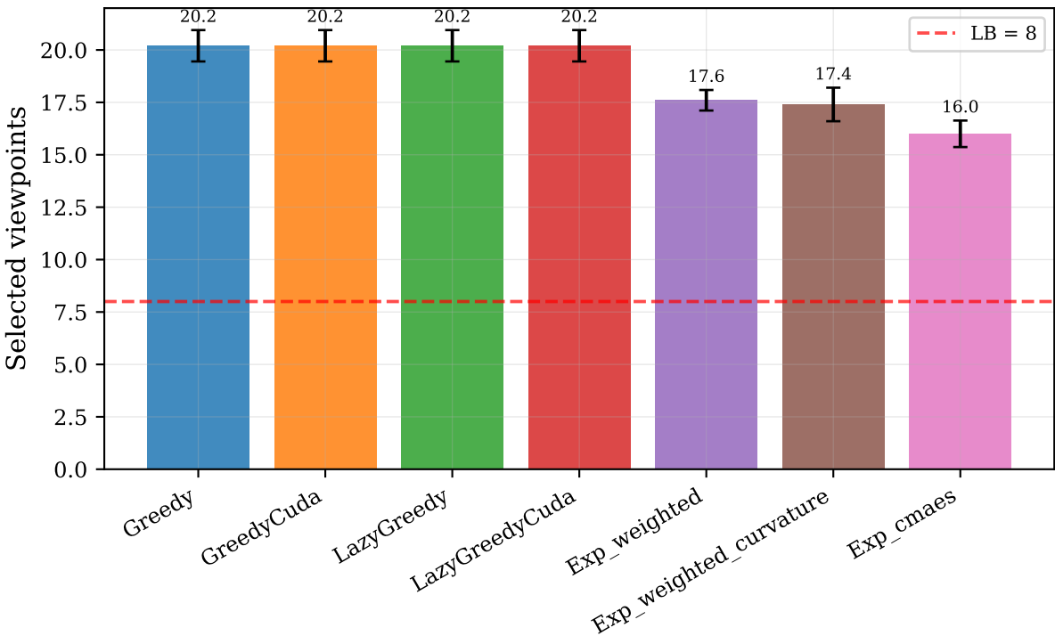
Viewpoints at 95% (david0)
