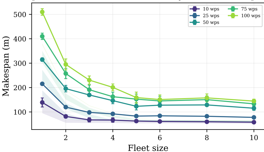
Makespan vs. Fleet Size (shaded: analytical LB band, per-seed)
