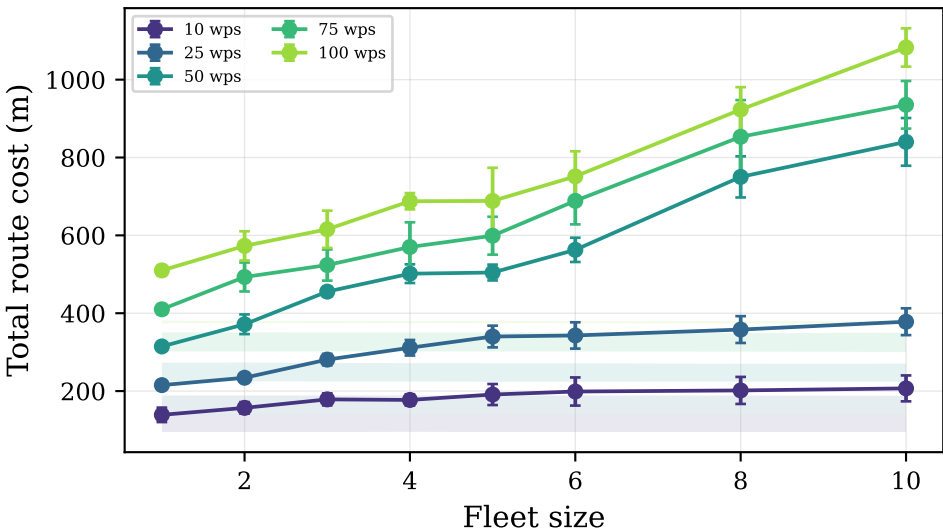
Total Cost vs. Fleet Size (shaded: analytical LB band, per-seed)
