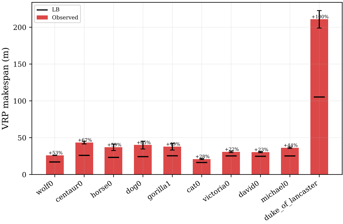
VRP Makespan by Model (K=5, \alpha=0.5 )
