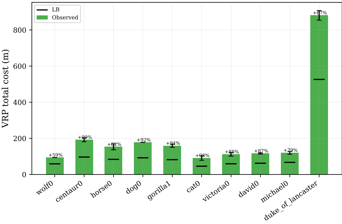
VRP Total Cost by Model (K=5, \alpha=0.5 )
