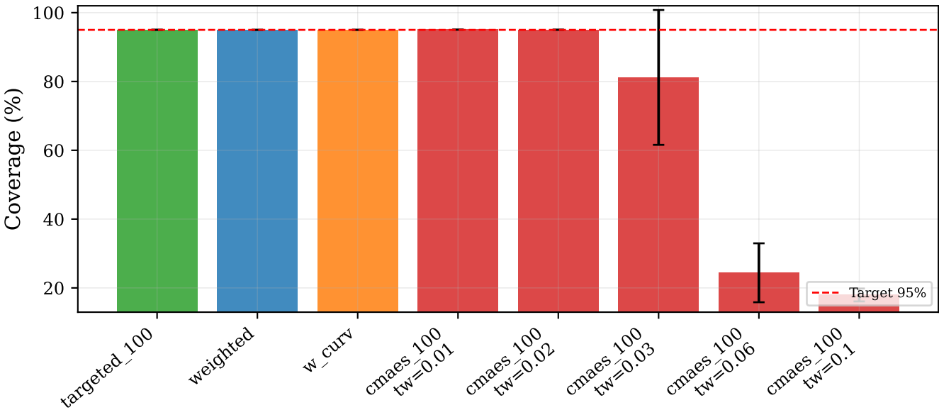
Coverage by Sampler Strategy
