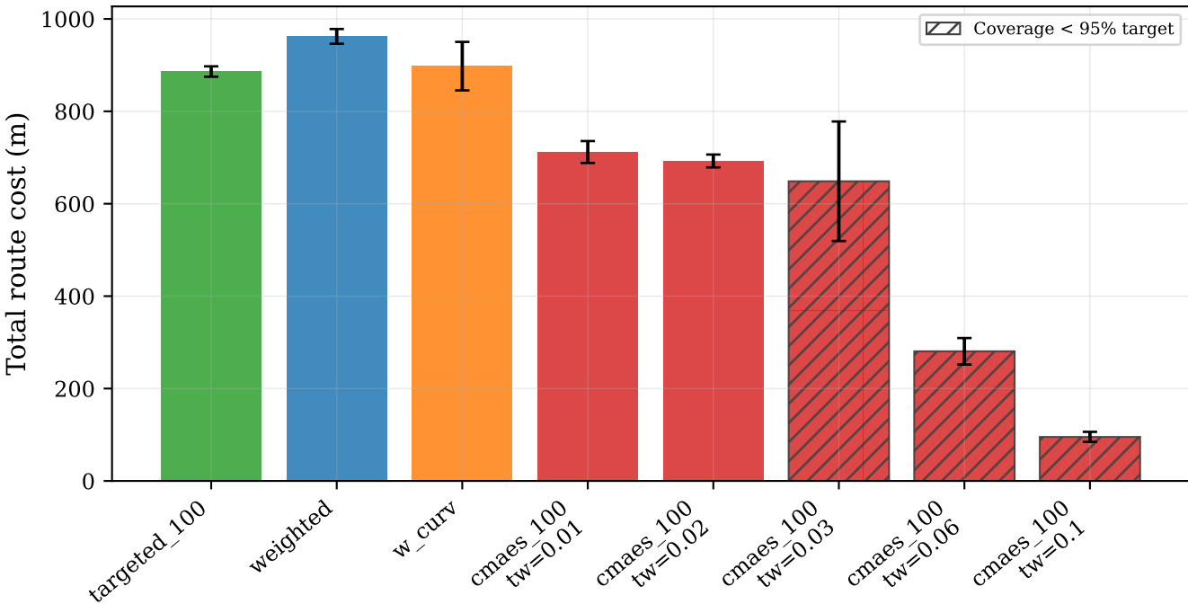
VRP Total Cost by Sampler Strategy
