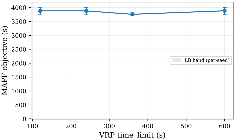
MAPF Objective vs VRP Time Limit
