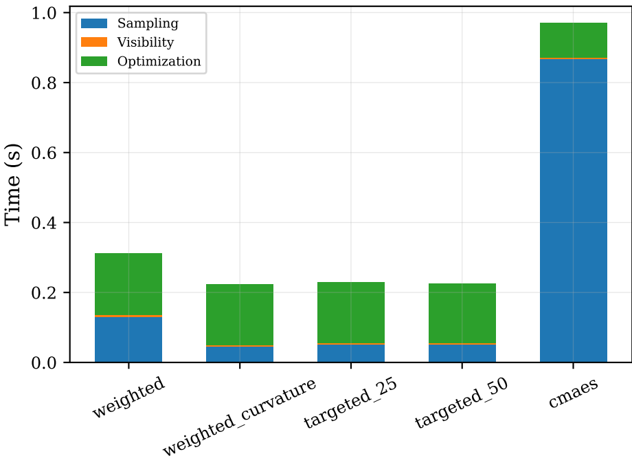
Time Breakdown (wolf0)
