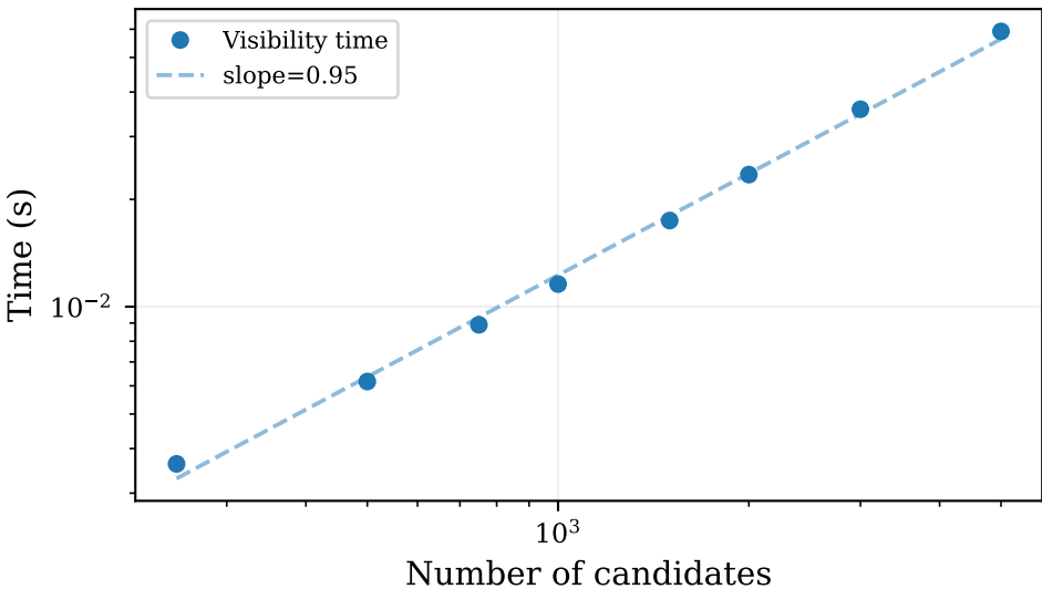
Visibility Computation Time (log-log)
