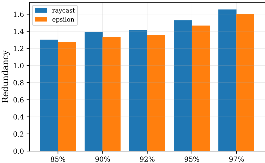
Redundancy (cat0)
