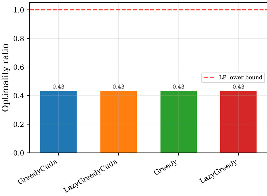
Optimality Ratio at 95% (david0)
