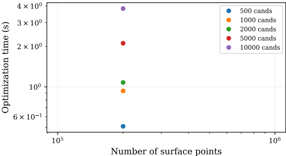
Set Cover Scaling (points)
