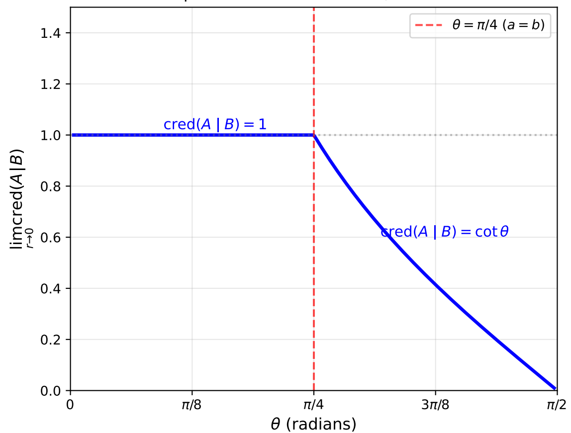
Path-dependent limit: \theta < \pi/4 \Rightarrow 1 , \theta > \pi/4 \Rightarrow \cot \theta
