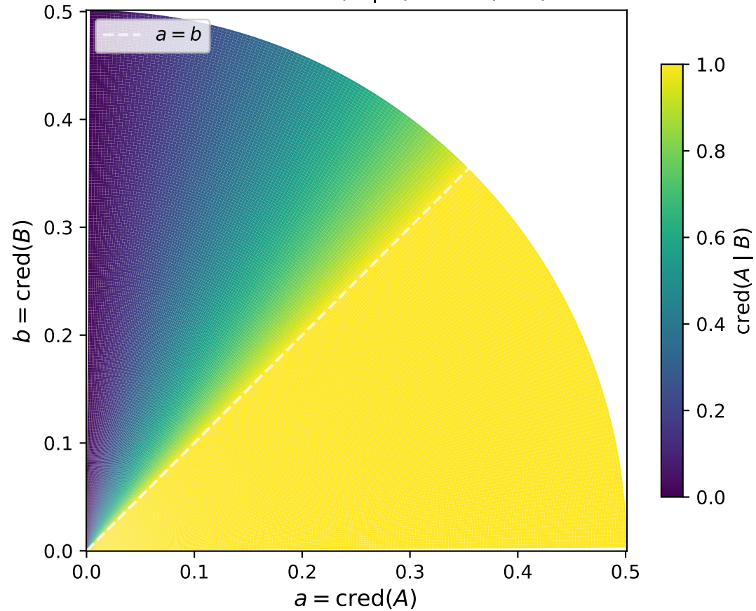
Conditional cred( A \mid B ) = \min(a, b)/b
