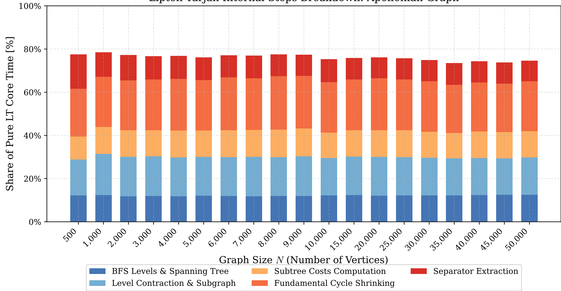
Lipton-Tarjan Internal Steps Breakdown: Apollonian Graph
