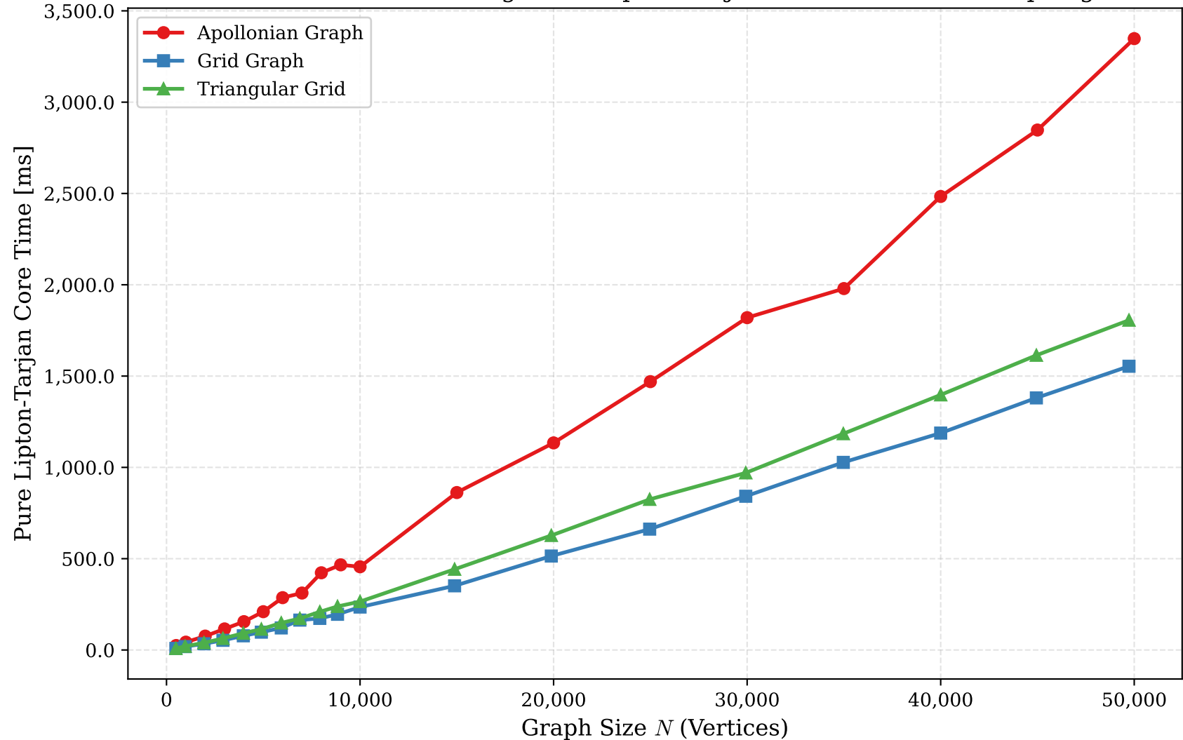
Planar Maximum Matching: Pure Lipton-Tarjan Core Time Across Topologies
