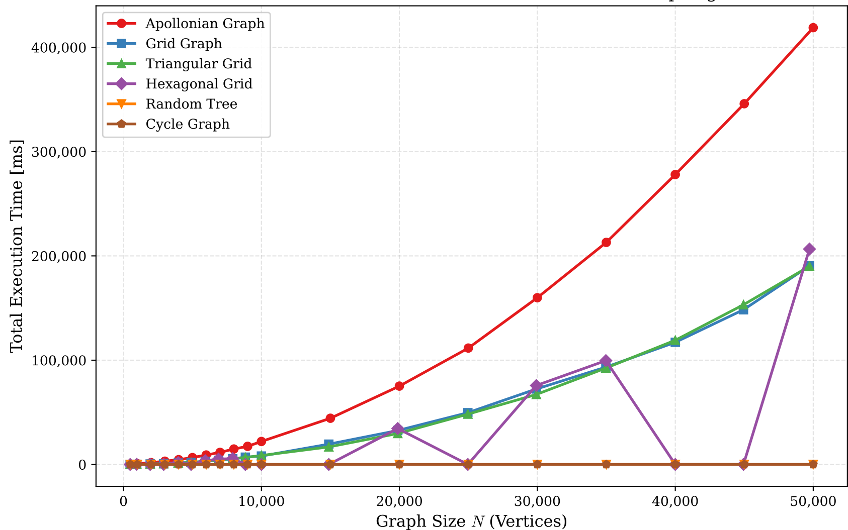
Planar Vertex Cover: Total Execution Time Across Topologies
