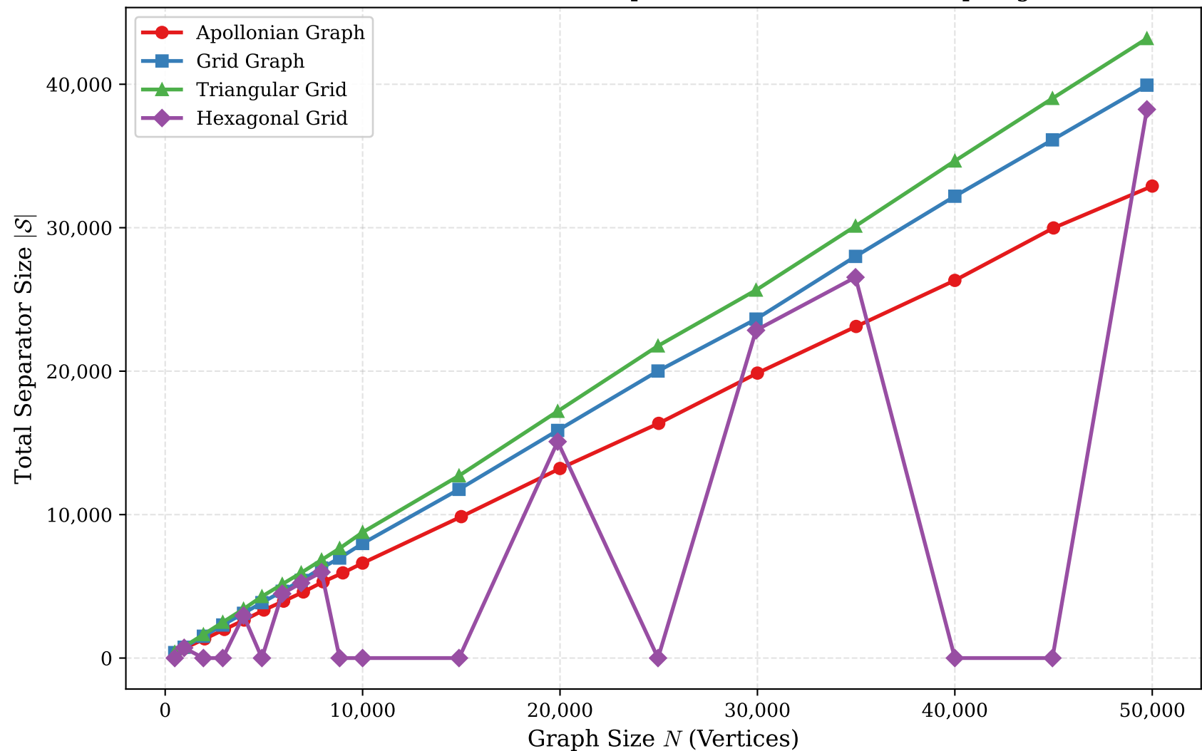
Planar Vertex Cover: Total Separator Vertices Across Topologies
