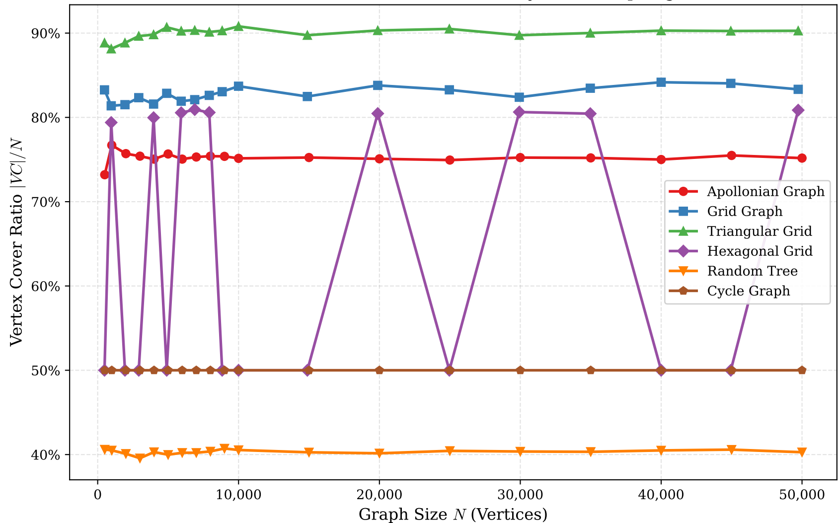
Planar Vertex Cover: Solution Density Across Topologies
