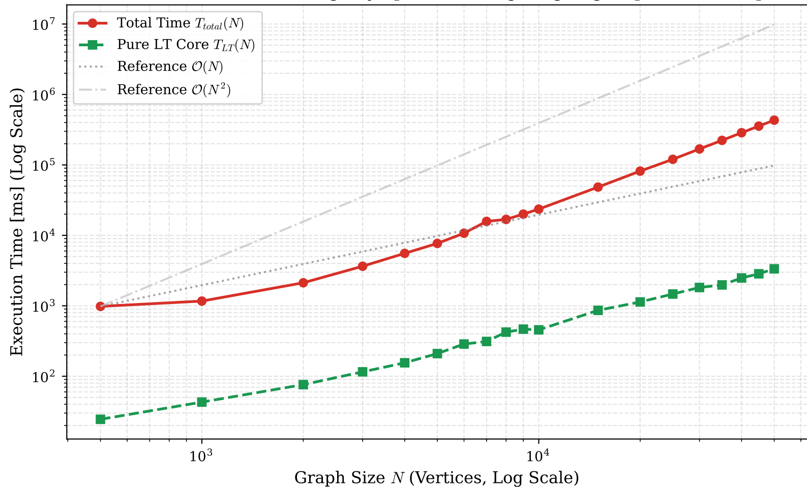
Planar Maximum Matching Asymptotic Scaling (Log-Log): Apollonian Graph
