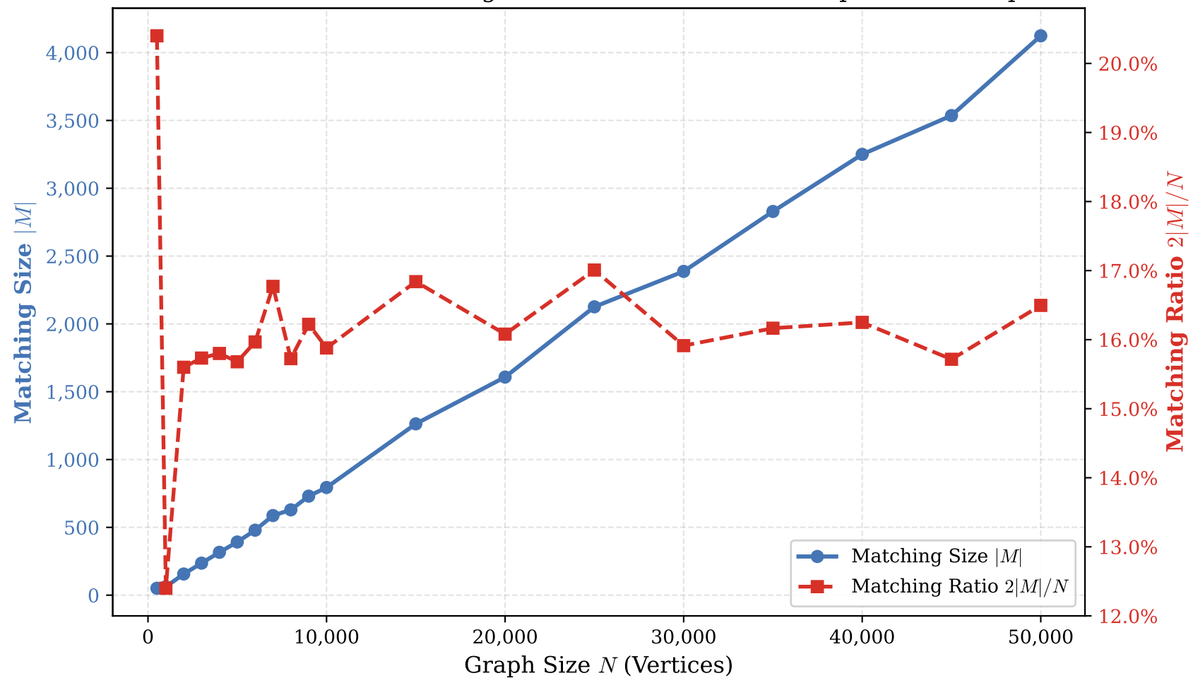
Planar Maximum Matching Solution Characteristics: Apollonian Graph
