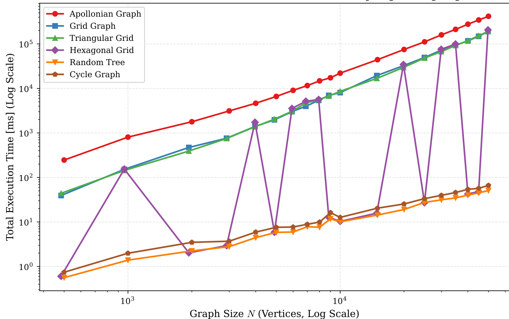
Planar Vertex Cover: Total Execution Time Across Topologies (Log-Log)
