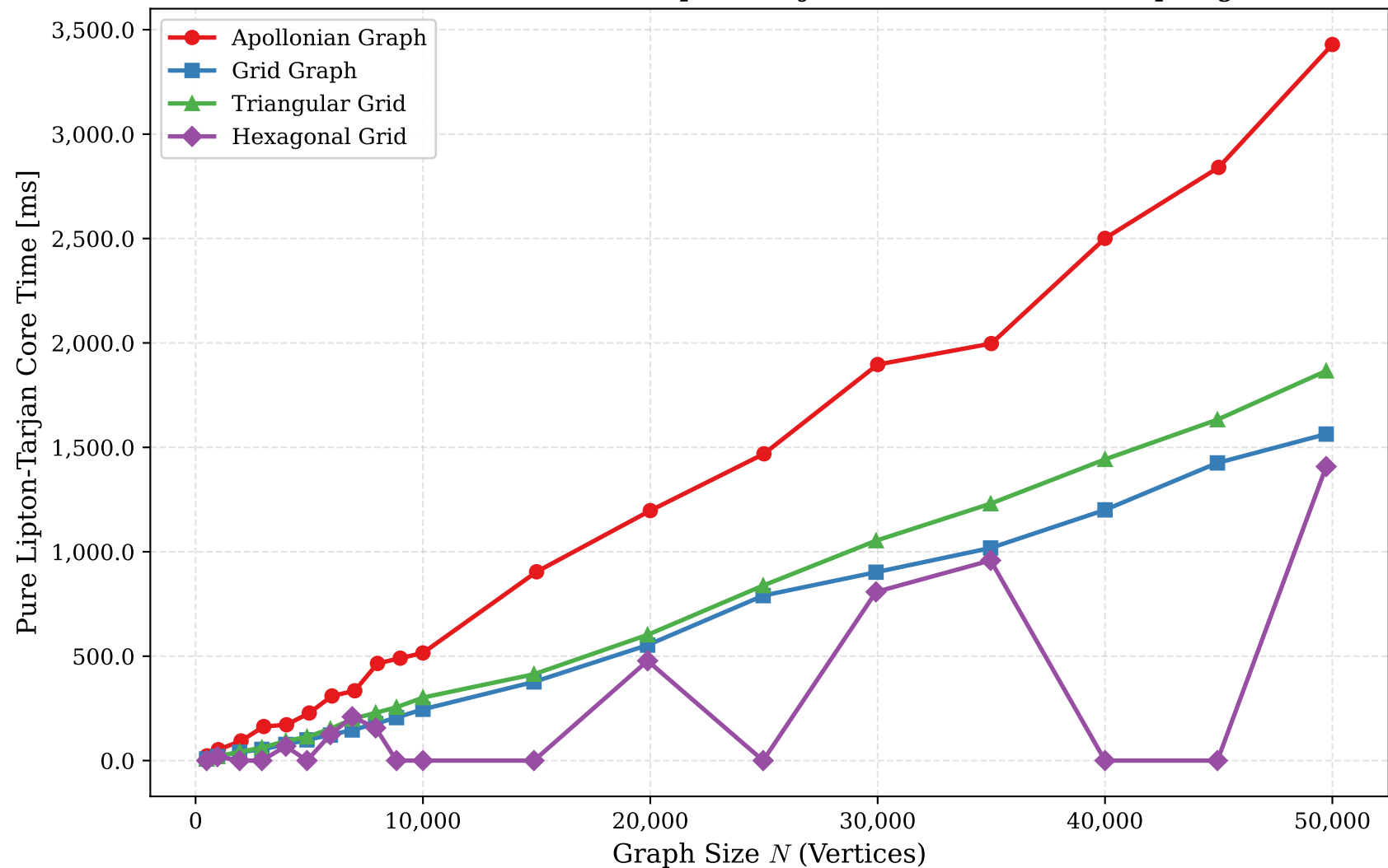
Planar Vertex Cover: Pure Lipton-Tarjan Core Time Across Topologies
