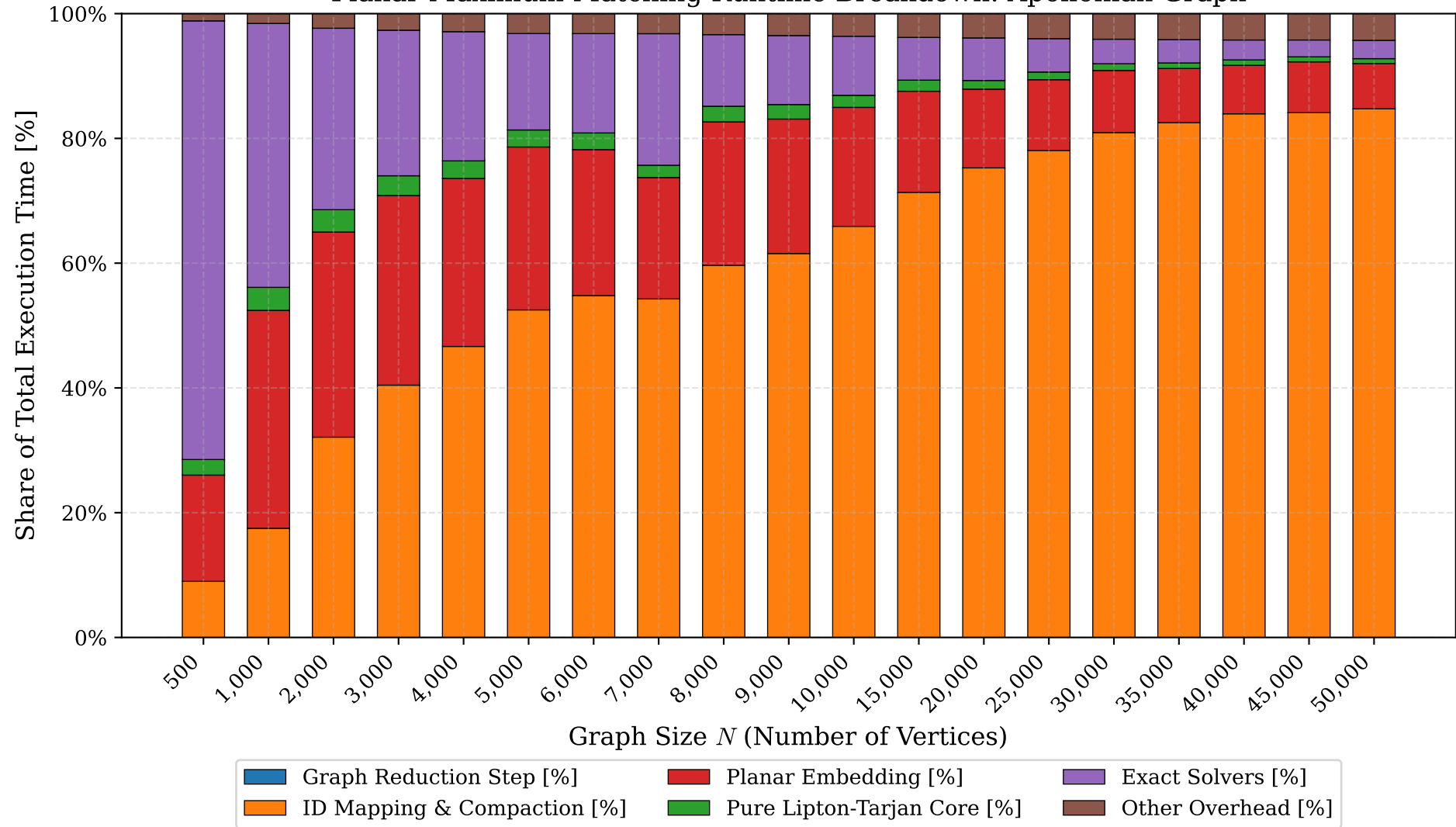
Planar Maximum Matching Runtime Breakdown: Apollonian Graph
