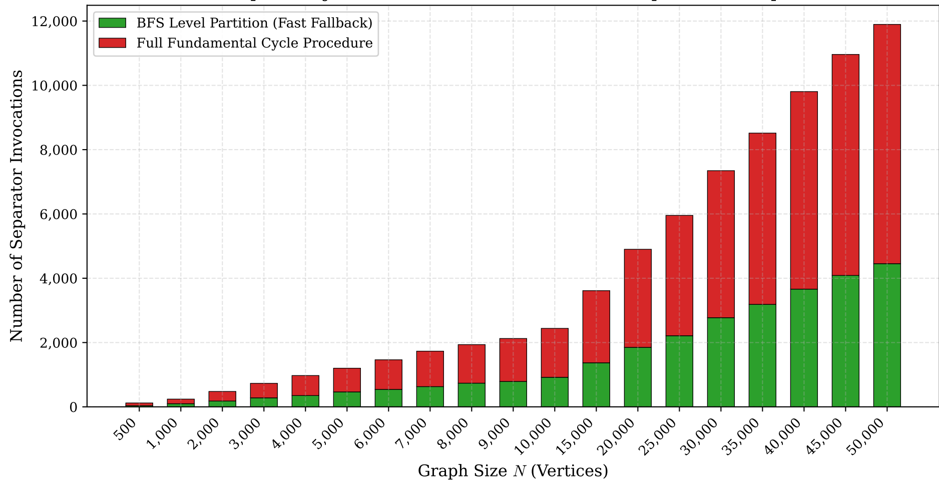
Lipton-Tarjan Path Distribution (Fast vs Full): Apollonian Graph
