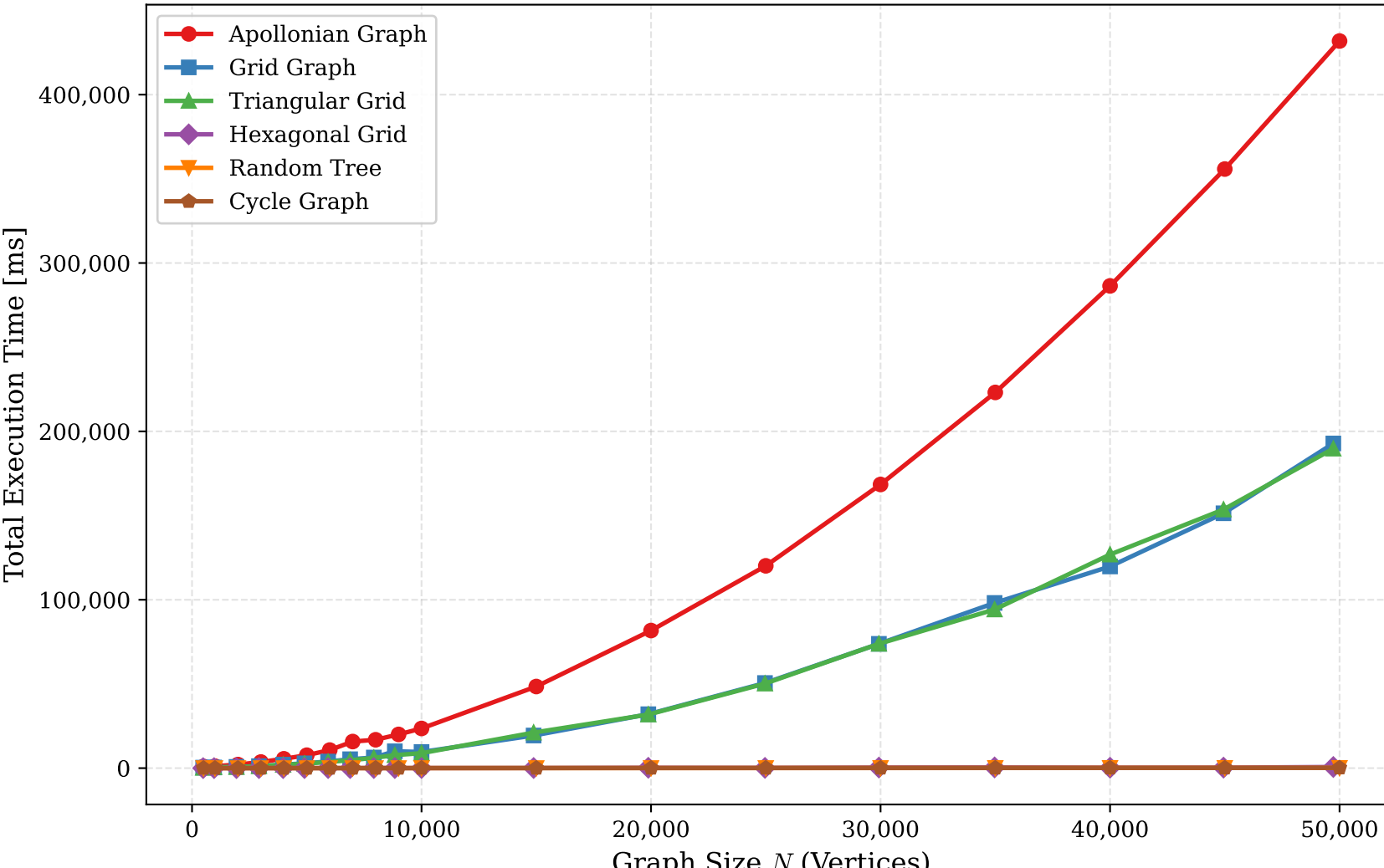
Planar Maximum Matching: Total Execution Time Across Topologies
