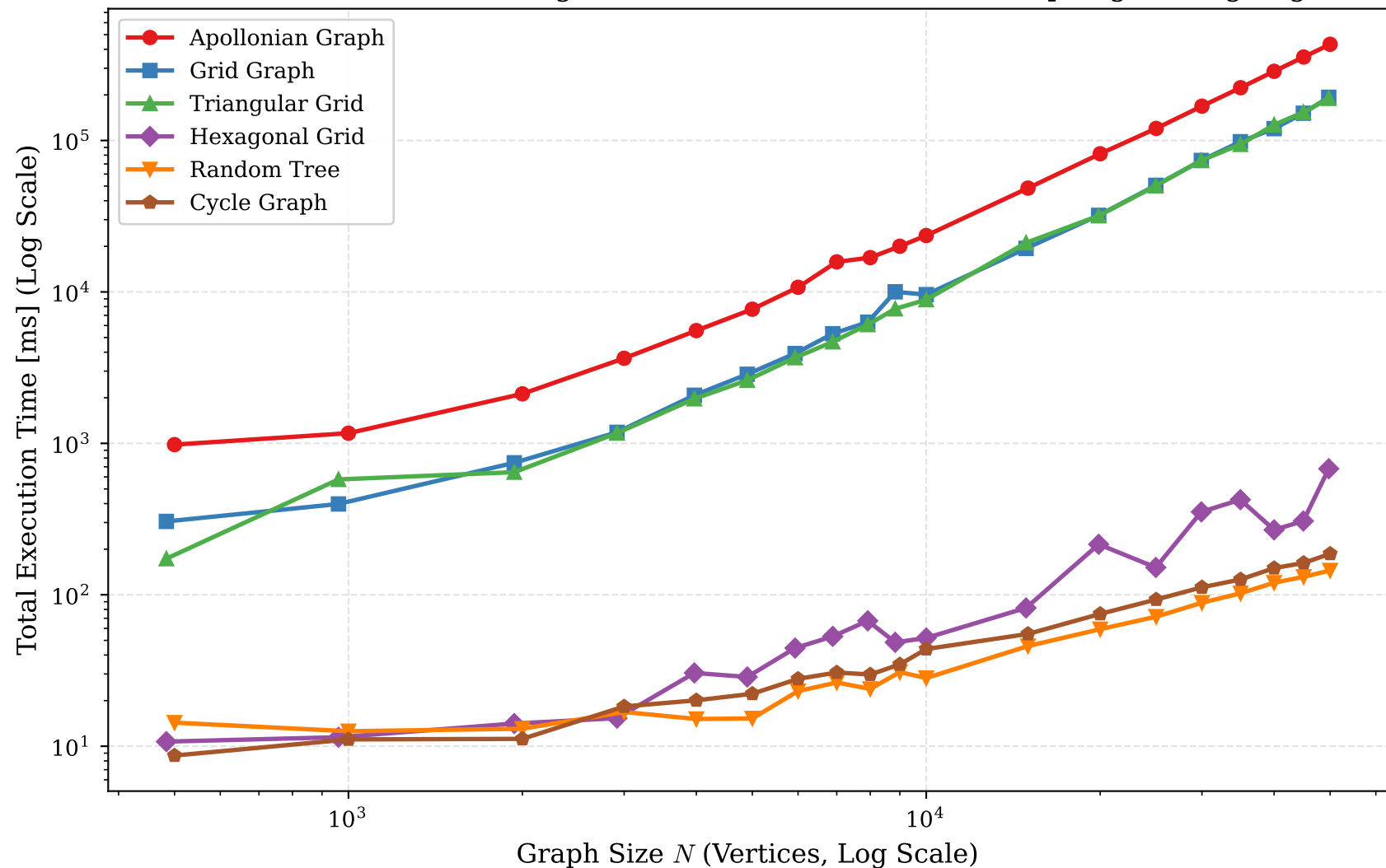
Planar Maximum Matching: Total Execution Time Across Topologies (Log-Log)
