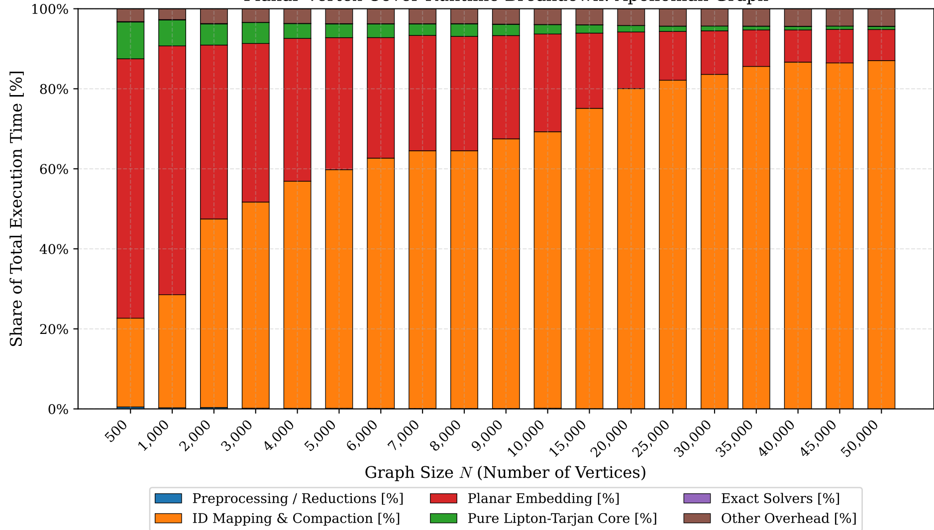
Planar Vertex Cover Runtime Breakdown: Apollonian Graph
