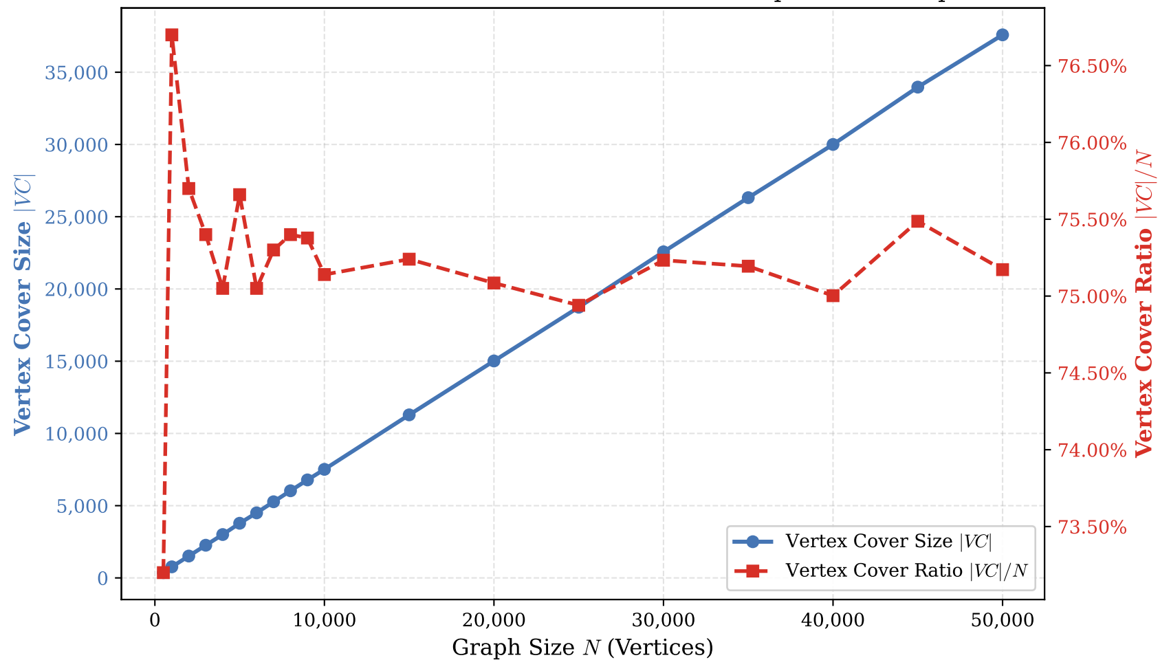
Planar Vertex Cover Solution Characteristics: Apollonian Graph
