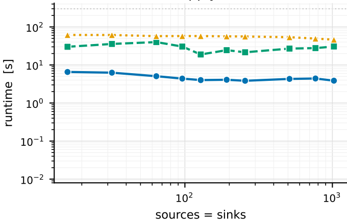
NETGEN — # supply/demand nodes
