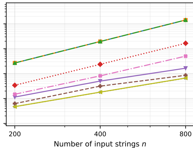
Phage lambda DNA, reads of length 100
