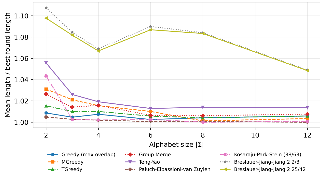
Superstring length ratio vs. alphabet size ( n = 20 )
