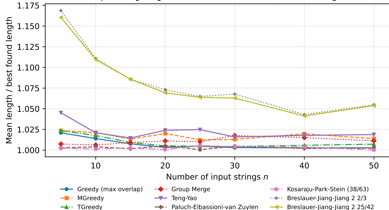
Superstring length ratio vs. instance size (random strings)
