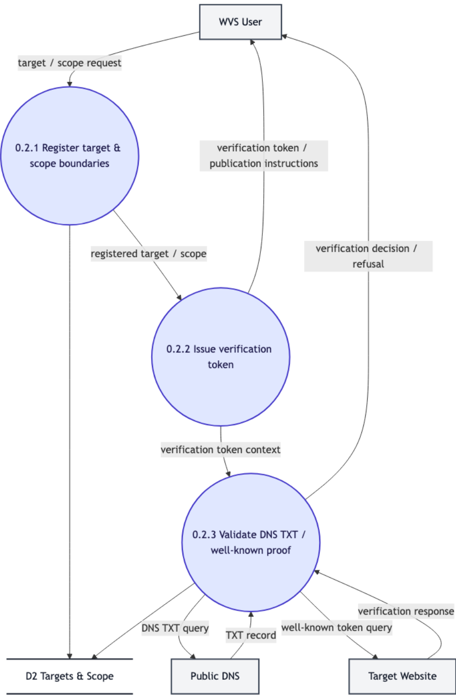
Figure 4: Level 2 DFD for 0.2 Target Management & Authorisation
