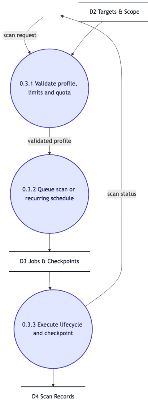
Figure 5: Level 2 DFD for 0.3 Scan Configuration & Execution
