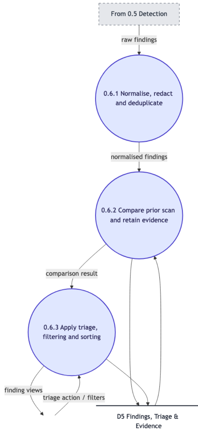
Figure 8: Level 2 DFD for 0.6 Findings Management
