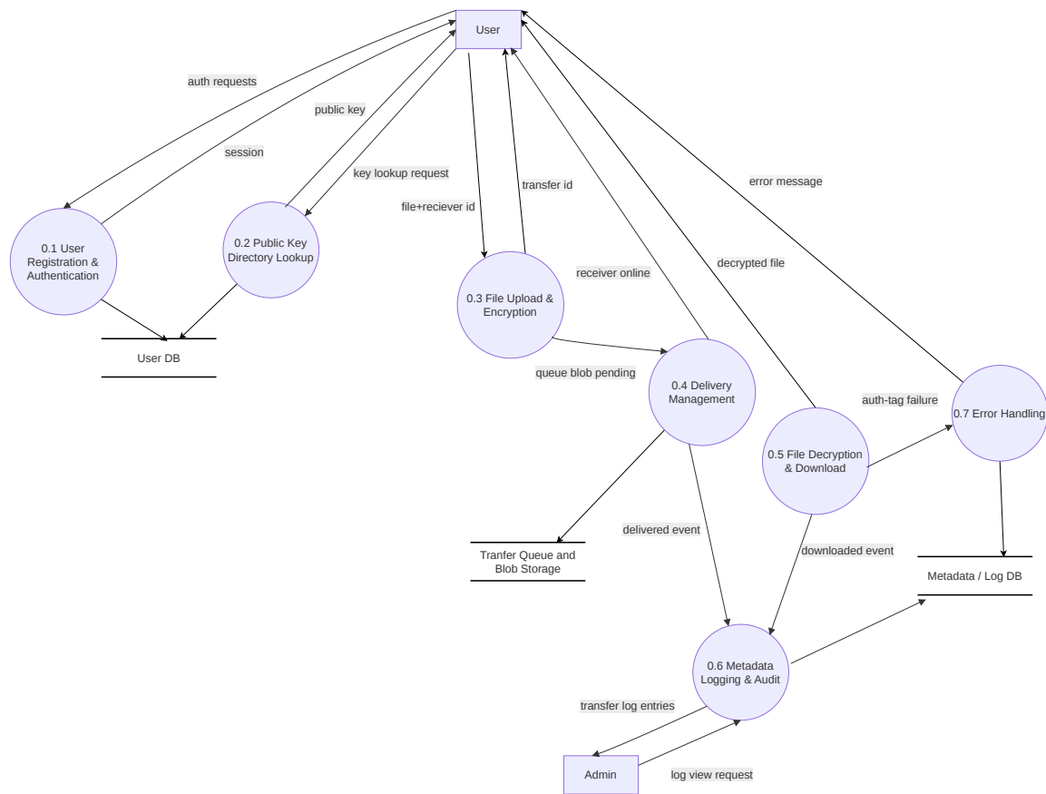
Figure 2: Level 1 DFD – process 0 decomposed into 7 functional groups
