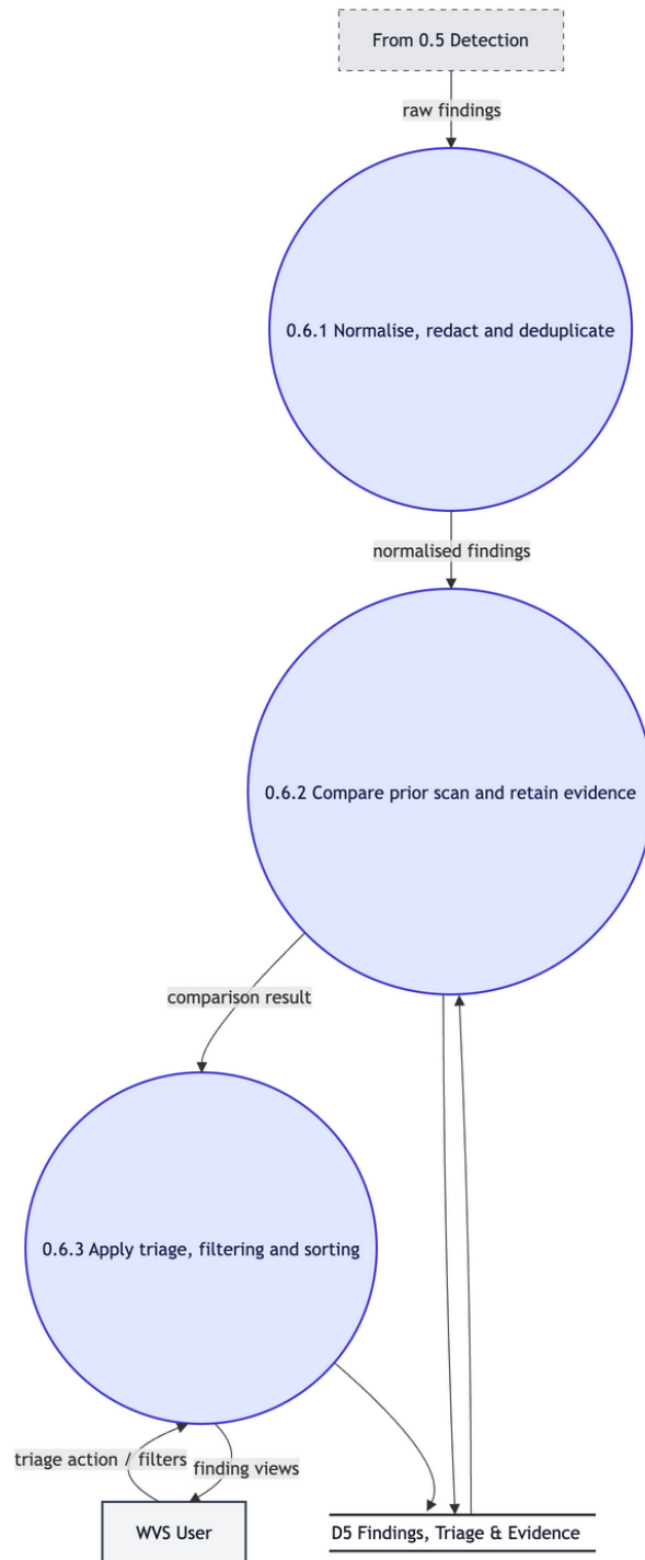
Figure 8: Level 2 DFD for 0.6 Findings Management
